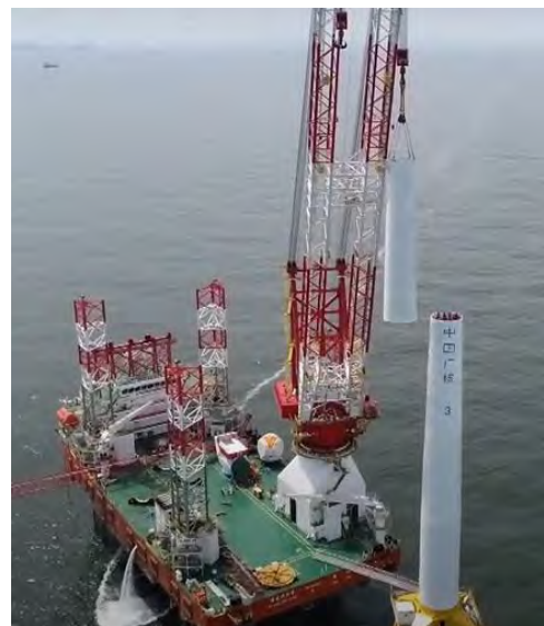
Figure 6-12: WTG assembly offshore [64]
